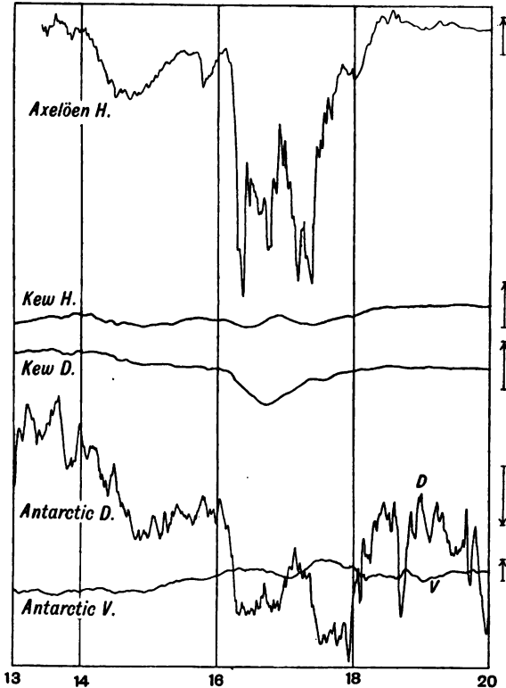
FIG. 40.—ARCTIC-KEW-ANTARCTIC CURVES.
